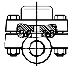
Steam trap plus pipe connector ( See IS 1.0915 and IS 1.0970 )
